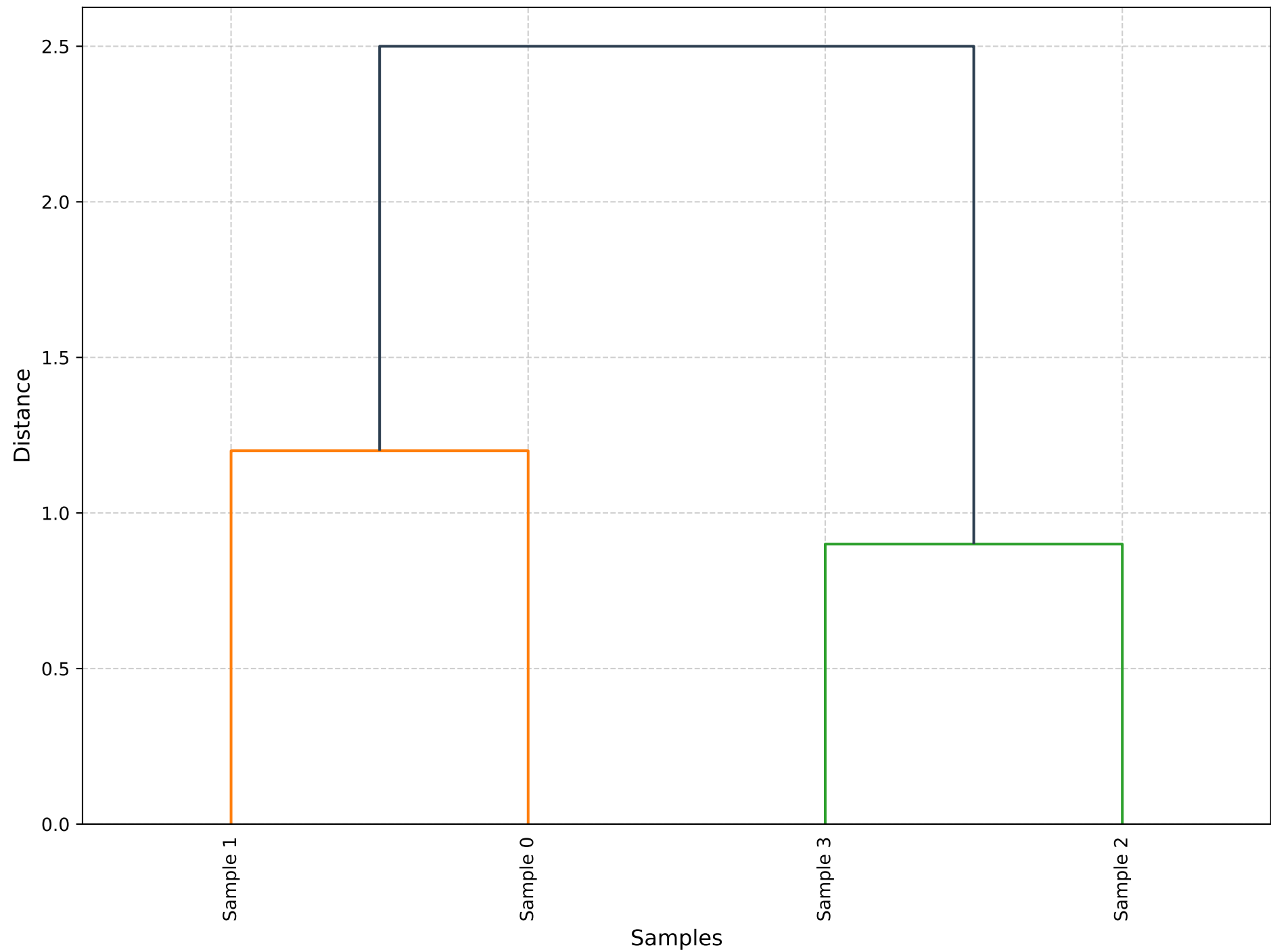
Rectangular Dendrogram
