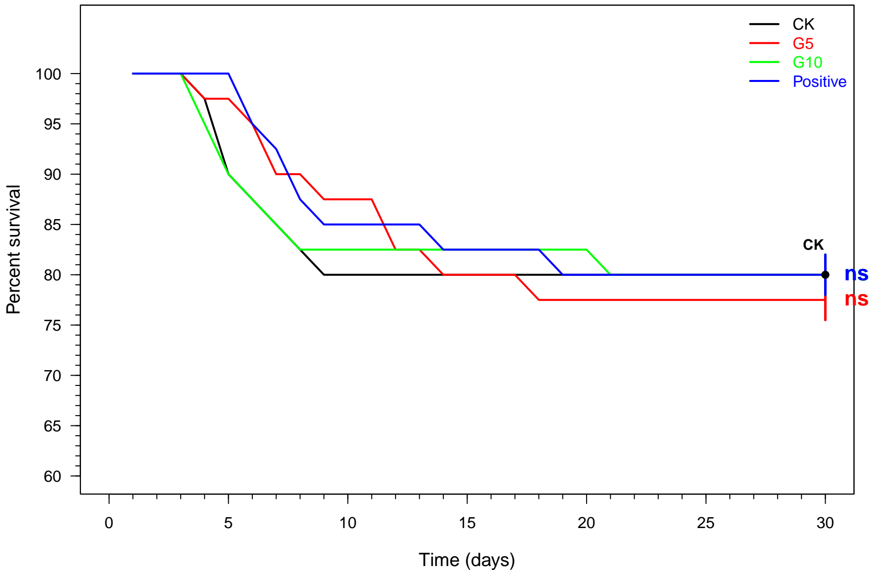
Fig. 1. Total survival of H. axyridis exposed to glyphosate.
